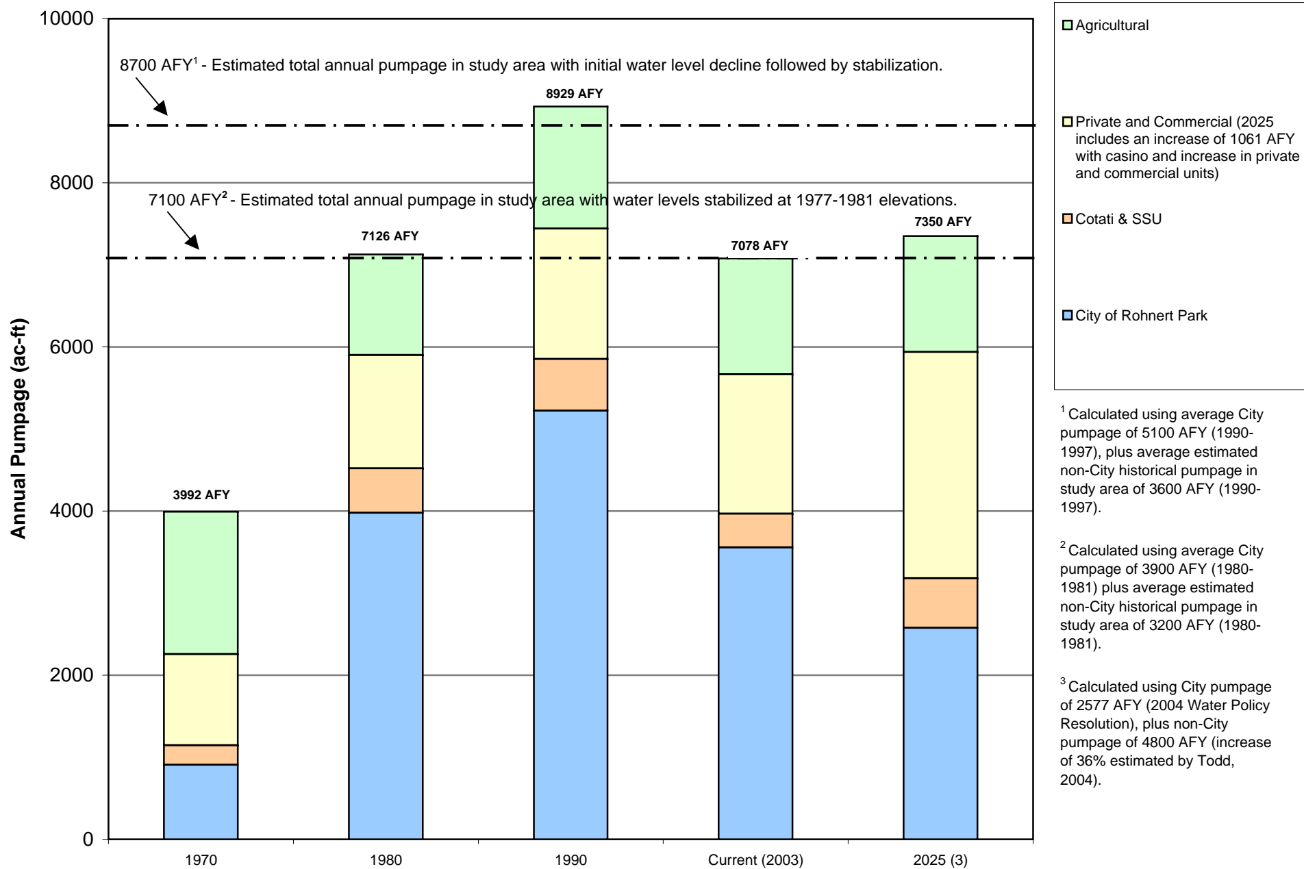
Figure 3-35 Historical, Current, and Future Annual Groundwater Pumpage with Increase in Future Non-City Pumpage in Study Area City of Rohnert Park WSA
